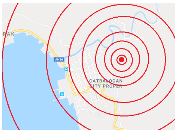
Figure 2. Location of Earthquake
