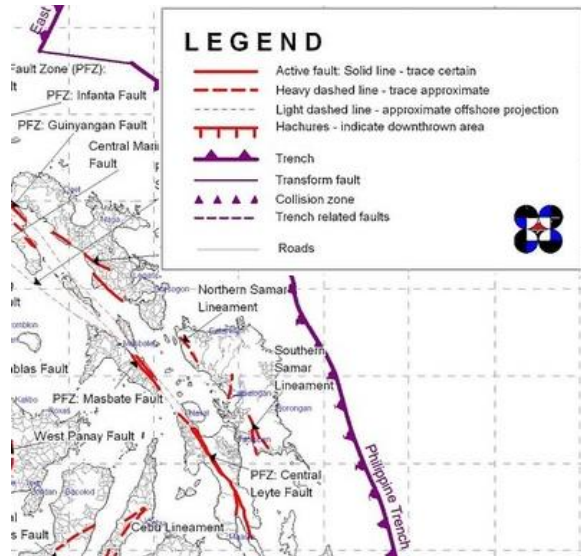
Figure 3. Distribution of Active Faults
