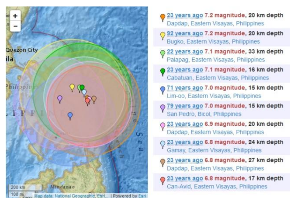
Figure 4. Biggest Earthquakes Near Samar, Philippines. (Source: Earthquake Track)
